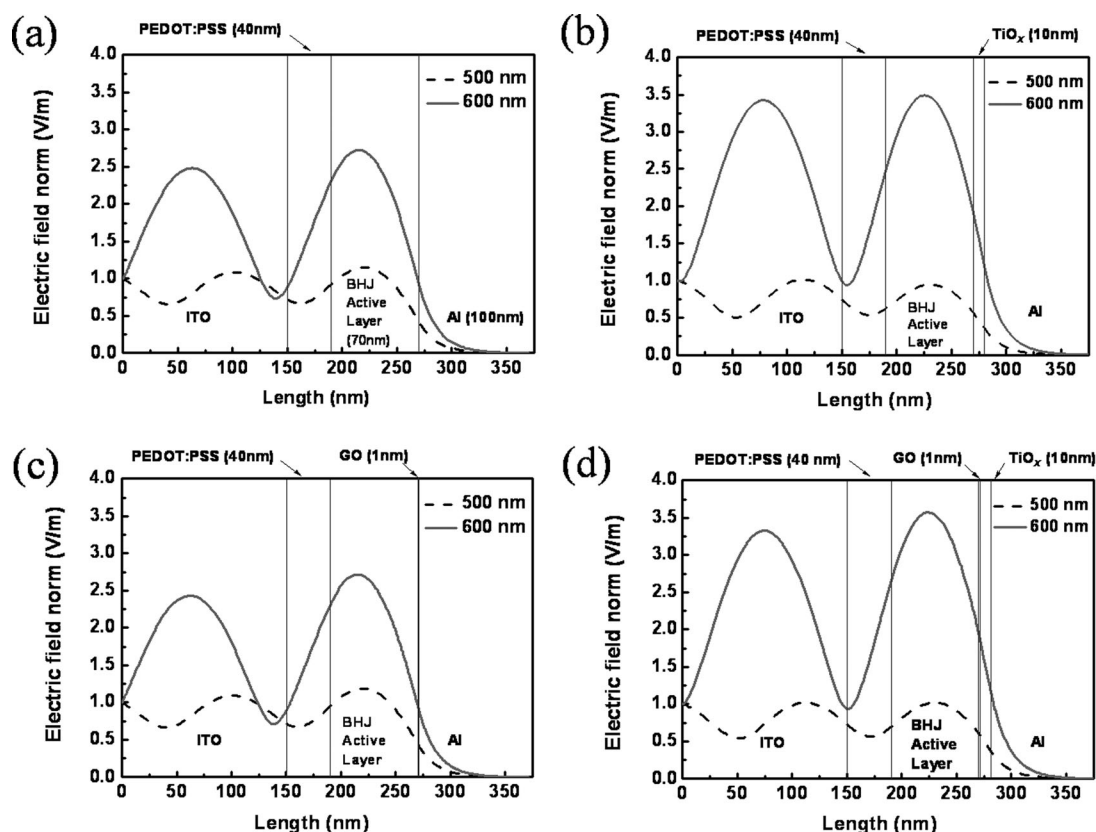
Figure 5. Simulated distribution of the normalized optical electric field for light inside BHJ devices as a function of wavelength: glass-ITO (150 nm)//PEDOT:PSS (40 nm)//PCDTBT:PC 71 BM BHJ (70 nm)//ETL//Al (100 nm), a) without ETL, b) with TiO x ( \approx 10 nm), c) with GO ( \approx 1 nm), d) with GO/TiO x ( \approx 11 nm).
